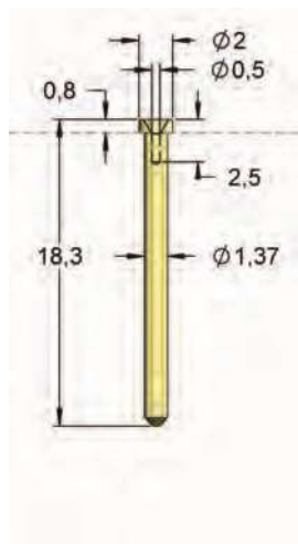
I-Z1S2 15,0 Ampères
