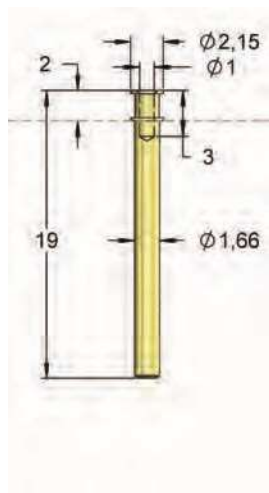
I-D19S1/2 15,0 Ampères
